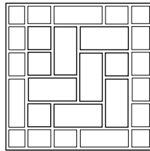
Cobblestone Pattern 32 pcs. per 100 s/f 12 x 24 67% 21 pcs. per 100 s/f 12 x 12 33%
