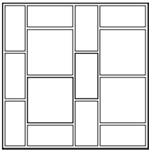
Corridor Pattern 17 pcs. per 100 s/f 24 x 24 67% 17 pcs. per 100 s/f 12 x 24 33%
